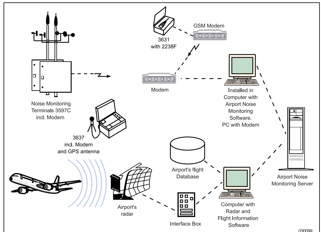
Fig. 1 Overview showing a complete airport-noise monitoring system setup. Noise-monitoring terminals are the heart of a complete, noise-monitoring installation
